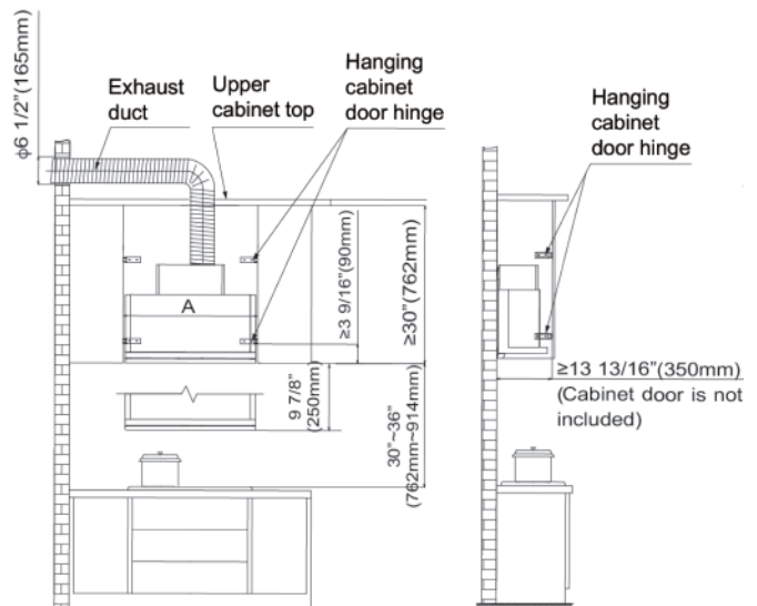
▼ Installation Dimensions
